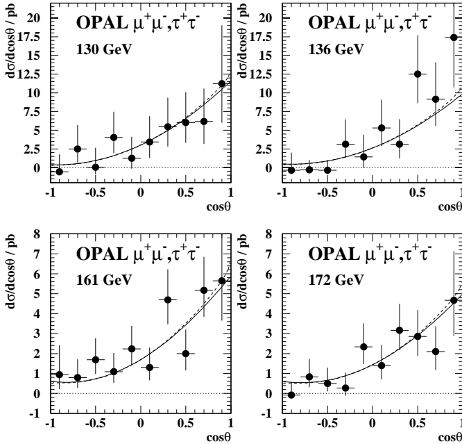
Fig. 14. Angular distributions for \mu^+\mu^- and \tau^+\tau^- events with s'/s > 0.8 . The data points show the measurements, which have been formed as a weighted average of the \mu^+\mu^- and \tau^+\tau^- distributions corrected to no interference between initial- and final-state radiation. The curves show the predictions of the ZFITTER program with no interference between initial- and final-state radiation ( solid ) and with interference ( dashed )
