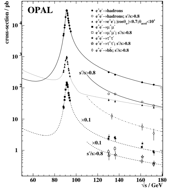
Fig. 10. Measured total cross-sections ( s'/s > 0.01 ) for different final states at lower energies [36,43,44], and this analysis. Cross-section measurements for hadrons, b\bar{b} , muon and tau pairs for s'/s > 0.8 from this analysis are also shown. The cross-sections for \mu^+\mu^- and \tau^+\tau^- production have been reduced by a factor of ten for clarity. The curves show the predictions of ZFITTER for hadronic ( solid ), b\bar{b} ( dot-dashed ), \mu^+\mu^- and \tau^+\tau^- ( dashed ) final states and that of ALIBABA for the e^+e^- final state ( dotted )
