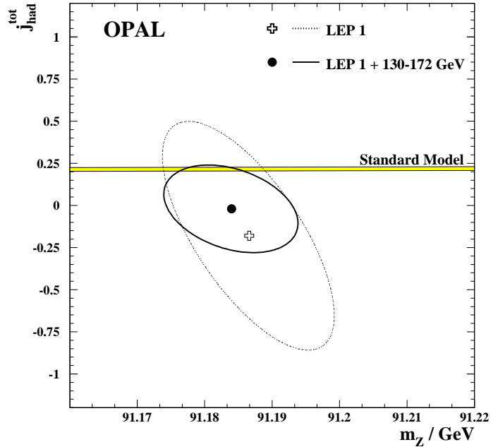
Fig. 16. Central values and one standard deviation contours (39% probability content) in the j_{\text{had}}^{\text{tot}} vs. m_Z plane resulting from model-independent fits to the OPAL data samples described in Sect. 4.1. The horizontal band shows the Standard Model expectation j_{\text{had}}^{\text{tot}} = 0.216 \pm 0.011 for a top quark mass of 175 \pm 5 GeV and a Higgs mass range of 70–1000 GeV
