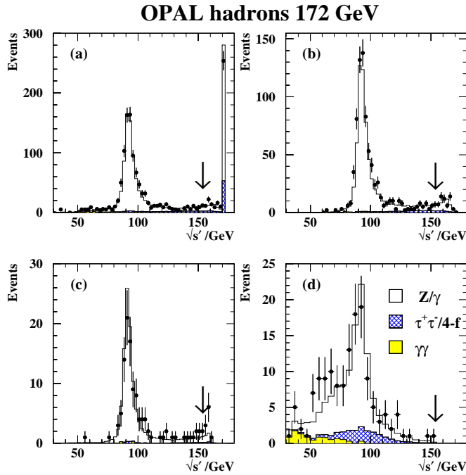
Fig. 3. Distributions of effective centre-of-mass energy \sqrt{s'} reconstructed for hadronic events at 172 GeV. The distributions are shown a for all events, b for events with one photon along the beam axis, c for events with one photon in the electromagnetic calorimeter and d for events with more than one photon. In each case the points show the data and the histogram the Monte Carlo prediction normalized to the luminosity of the data. The arrows indicate the position of the cut used to select ‘non-radiative’ events
