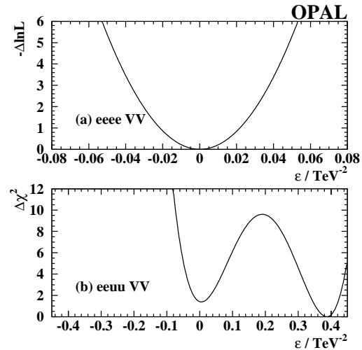
Fig. 20. a Negative log likelihood curve for the contact interaction fit to the e^+e^- angular distribution for the VV model. b \chi^2 curve for the contact interaction fit to the hadronic cross-section, assuming coupling to only one up-type quark, for the same model
