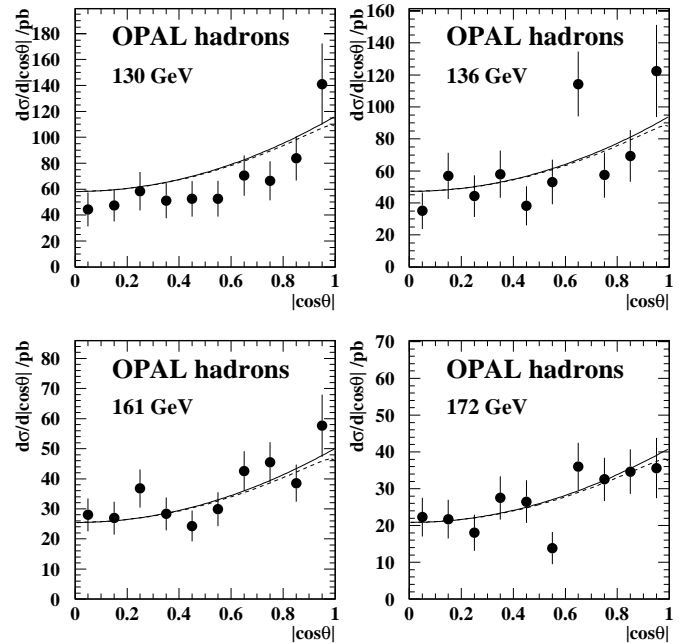
Fig. 12. Angular distributions for hadronic events with s'/s > 0.8 . The data points show the measurements corrected to the direction of the primary quark/antiquark, and corrected to no interference between initial- and final-state radiation. The curves show the predictions of the ZFITTER program with no interference between initial- and final-state radiation ( solid ) and with interference ( dashed )
