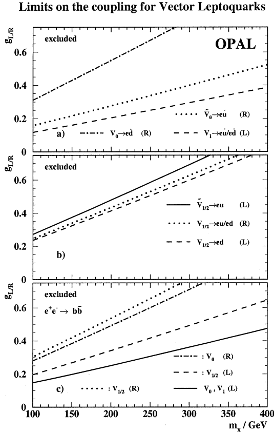
Fig. 22. 95% confidence exclusion limits on g_L or g_R as a function of m_X , for various possible vector leptoquarks. a and b show limits on leptoquarks coupling to a single quark family, derived from the hadronic cross-sections. c shows limits on leptoquarks coupling to b quarks only, derived from the b\bar{b} cross-sections. The excluded regions are above the curves in all cases. The letter in parenthesis after the different leptoquark types indicates the chirality of the lepton involved in the interaction
