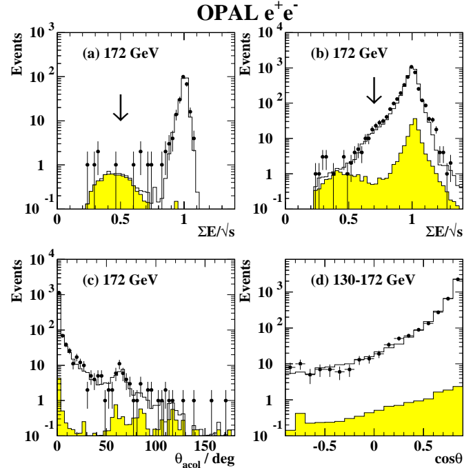
Fig. 4. a The distribution of the ratio of total electromagnetic calorimeter energy to the centre-of-mass energy for e^+e^- \rightarrow e^+e^- events in acceptance region B, |\cos\theta_{e^-}| < 0.7 and \theta_{\text{acol}} < 10^\circ , at 172 GeV. b The same distribution for the large acceptance selection, C, |\cos\theta| < 0.96 and \theta_{\text{acol}} < 10^\circ , at 172 GeV. Distributions are shown after all cuts except the one on total electromagnetic calorimeter energy; the arrows indicate the positions of the cuts on this quantity. c The acollinearity angle distribution for events satisfying the inclusive selection, in the acceptance region A, |\cos\theta_{e^+}| < 0.9 , |\cos\theta_{e^-}| < 0.9 , at 172 GeV. The cut on acollinearity angle has not been applied. d Observed distribution of \cos\theta of the outgoing electron in e^+e^- events with \theta_{\text{acol}} < 10^\circ . All centre-of-mass energies have been summed for this plot. In each case, the points show the data and the histograms the Monte Carlo expectations, normalized to the integrated luminosity of the data, with the background contributions shaded
