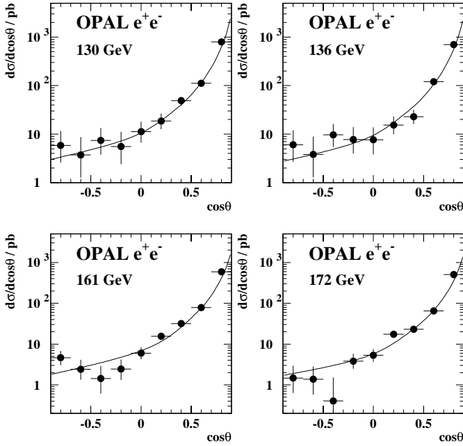
Fig. 13. Angular distributions for e^+e^- events with \theta_{\text{acol}} < 10^\circ . The points show the data, the curves the predictions of the ALIBABA program.
