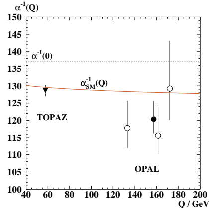
Fig. 17. Fitted values of 1/\alpha_{\text{em}} as a function of Q , which is \sqrt{s} for the OPAL fits. The open circles show the results of the fits at each centre-of-mass energy, the closed circle the result of the combined fit. The value obtained by the TOPAZ experiment [49] is also shown for comparison. The solid line shows the Standard Model expectation, with the thickness representing the uncertainty, while the value of 1/\alpha_{\text{em}}(0) is shown by the dashed line
