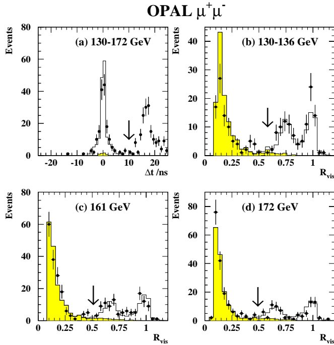
Fig. 6. a The time difference between hits in back-to-back TOF counters for muon pair candidates; data from all energies have been included in this figure. b The distribution of the ratio of the visible energy to the centre-of-mass energy for muon pair events at 130–136 GeV. c and d show similar distributions at 161 and 172 GeV. In each case, the points show the data and the histogram the Monte Carlo expectation, normalized to the integrated luminosity of the data, with the background contribution shaded. The arrows show the positions of the cuts, which for the R_{\text{vis}} distributions are positioned 0.15 below the expected value for radiative return events where the photon is undetected
