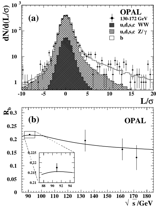
Fig. 9. a Decay length significance distribution for all centre-of-mass energies combined. The points show the data, the histogram the Monte Carlo prediction. b R_b as a function of the centre-of-mass energy. The points show the measurements presented here, and the value [41] obtained on the Z peak. The errors are statistical and systematic, summed in quadrature. The solid line is the ZFITTER prediction for s'/s > 0.8
