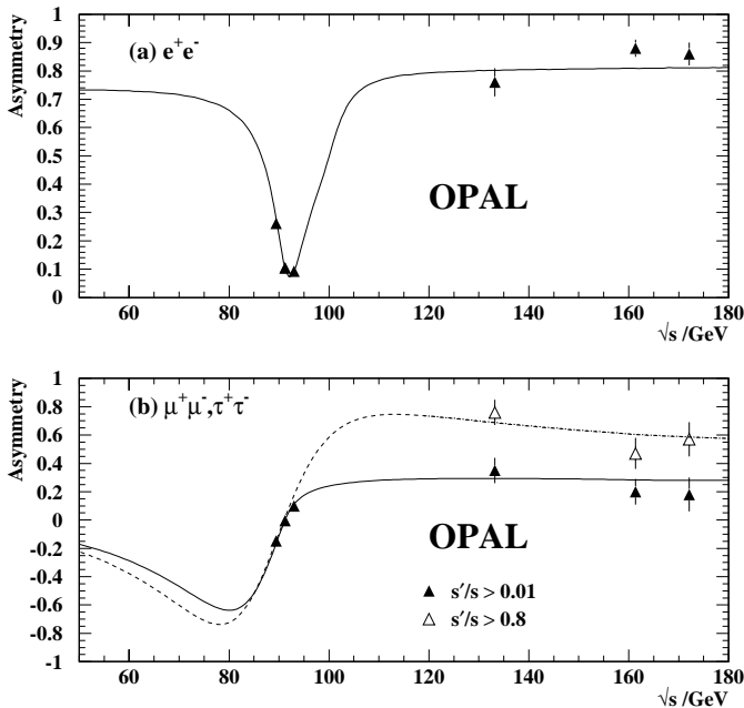
Fig. 11. a Measured forward-backward asymmetry for electron pairs with |\cos\theta_{e^-}| < 0.7 and \theta_{\text{acol}} < 10^\circ , as a function of \sqrt{s} . The curve shows the prediction of ALIBABA. b Measured asymmetries for all ( s'/s > 0.01 ) and non-radiative ( s'/s > 0.8 ) samples as functions of \sqrt{s} for \mu^+\mu^- and \tau^+\tau^- events (combined). The curves show ZFITTER predictions for s'/s > 0.01 ( solid ) and s'/s > 0.8 ( dotted ), as well as the Born-level expectation without QED radiative effects ( dashed ). The expectation for s'/s > 0.8 lies extremely close to the Born curve , such that it appears indistinguishable on this plot
