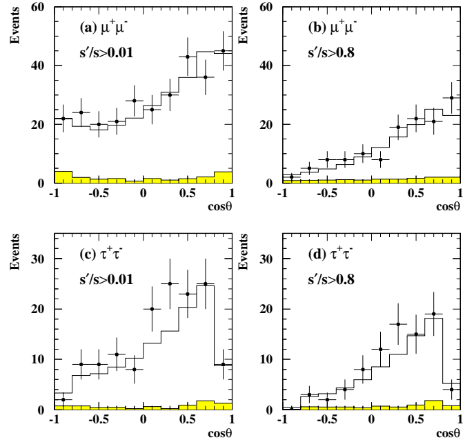
Fig. 7. Observed distributions of \cos\theta of the outgoing negative lepton in muon and tau pair events. a and b show muon pair events with s'/s > 0.01 and s'/s > 0.8 respectively, c and d tau pair events with s'/s > 0.01 and s'/s > 0.8 . The points show data for all energies combined, while the histograms show the Monte Carlo expectations, formed by summing the predictions at each energy normalized to the measured integrated luminosity values. The background contributions (including feedthrough from lower s' in the s'/s > 0.8 cases) are shaded
