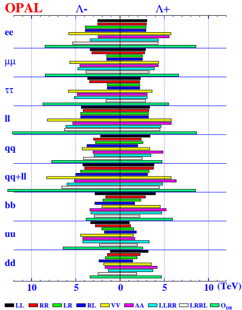
Fig. 19. 95% confidence level limits on the energy scale \Lambda resulting from the contact interaction fits. For each channel, the bars from top to bottom indicate the results for models LL to \overline{\mathcal{O}}_{\text{DB}} in the order given in the key
