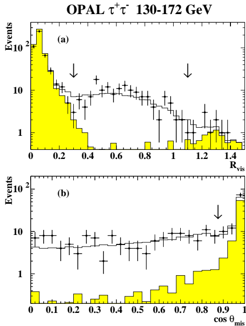
Fig. 8. a The distribution of the ratio of the visible energy to the centre-of-mass energy for tau pair events. Note that visible energy here is defined as the scalar sum of track momenta plus electromagnetic calorimeter energy, with no correction for double counting. b Distribution of \cos\theta of the missing momentum vector, calculated using electromagnetic clusters, for tau pair candidates. Data from all energies have been included in this figure. In each case, the points show the data and the histogram the Monte Carlo expectation, normalized to the integrated luminosity of the data, with the background contribution shaded. The arrows show the positions of the cuts
