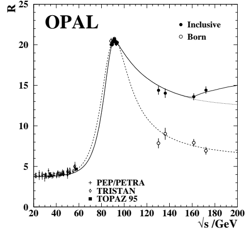
Fig. 15. Ratio of measured hadronic cross-sections to the theoretical muon pair cross-sections as a function of centre-of-mass energy. Values are shown for the inclusive cross-section, \sigma(q\bar{q}X) and for the Born level cross-section, as described in the text. The dotted and dashed curves show the predictions of ZFITTER for these cross-sections, while the solid curve also includes the contributions from W-pairs calculated using GENTLE and from Z-pairs calculated using FERMISV. Measurements at lower energies are from [36, 43, 44, 46]
