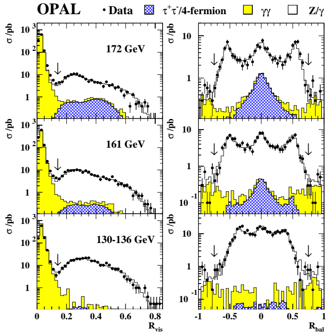
Fig. 2. The distributions of R_{\text{vis}} , the ratio of the total energy deposited in the electromagnetic calorimeter to the centre-of-mass energy, and R_{\text{bal}} , the energy imbalance along the beam direction, for hadronic events at each energy. Distributions are shown after all event selection cuts except the cut on that quantity. The positions of the cuts are indicated by the arrows . Points show the data and histograms the Monte Carlo expectations, normalized to the integrated luminosity of the data, with light shading indicating background from two-photon events and cross-hatching indicating other backgrounds, mainly four-fermion (including WW) and \tau^+\tau^- events
