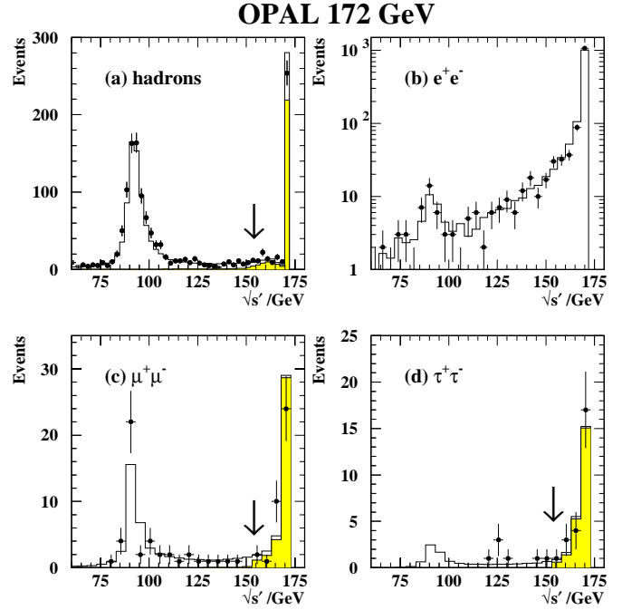
Fig. 5. The distributions of \sqrt{s'} for a hadronic events, b electron pair events with |\cos\theta_{e^+}| < 0.9 , |\cos\theta_{e^-}| < 0.9 and \theta_{acol} < 170^\circ , c muon pair and d tau pair events at 172 GeV. In each case, the points show the data and the histogram the Monte Carlo prediction, normalized to the integrated luminosity of the data, with the contribution from events with true s'/s > 0.8 shaded in a , c and d . The arrows in a , c and d show the position of the cut used to select ‘non-radiative’ events
