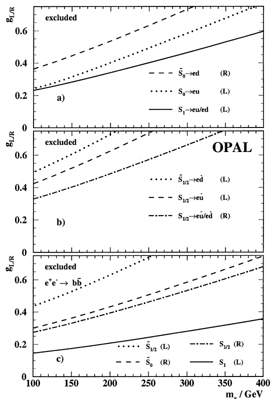
Fig. 21. 95% confidence exclusion limits on g_L or g_R as a function of m_X , for various possible scalar leptoquarks. a and b show limits on leptoquarks coupling to a single quark family, derived from the hadronic cross-sections. c shows limits on leptoquarks coupling to b quarks only, derived from the b\bar{b} cross-sections. The excluded regions are above the curves in all cases. The letter in parenthesis after the different leptoquark types indicates the chirality of the lepton involved in the interaction. The limits on the S_0 and \tilde{S}_{1/2} leptoquarks can be interpreted as those on R -parity violating \tilde{d}_R and \tilde{u}_L squarks respectively
