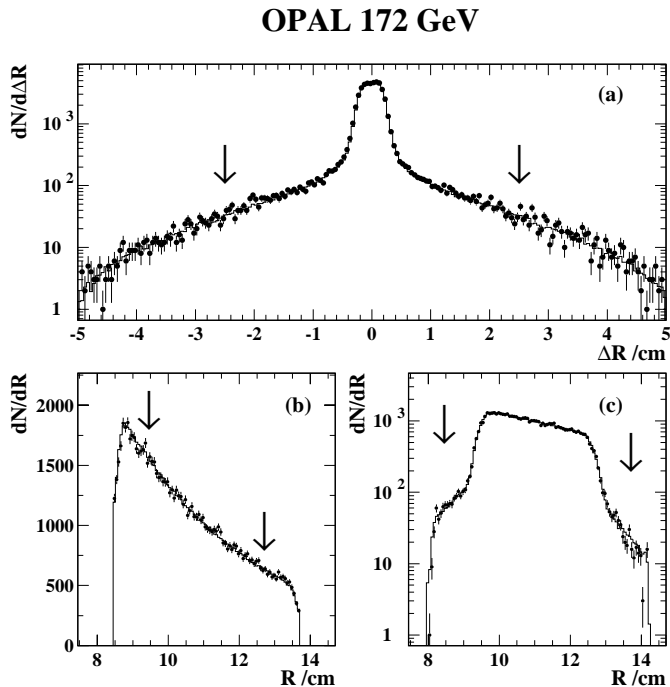
Fig. 1. a The distribution of the difference in radial coordinate between the two clusters in Bhabha scattering events used for the silicon-tungsten luminosity measurement at 172 GeV. Distributions of the radial coordinates of clusters for b the ‘narrow’ side and c the ‘wide’ side calorimeter. Distributions are shown after all cuts except the acollinearity cut in a and the inner and outer radial acceptance cuts, on that side, in b and c . Points show the data, while the histograms show the Monte Carlo expectation. The arrows show the positions of the cuts which define the acceptance
